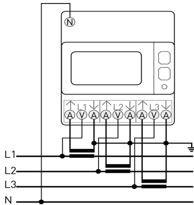
3 FASI, 4 FILI, 3 TA 3 PHASES, 4 WIRES, 3 CTs
