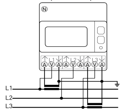
3 FASI, 3 FILI, 2 TA 3 PHASES, 3 WIRES, 2 CTs
